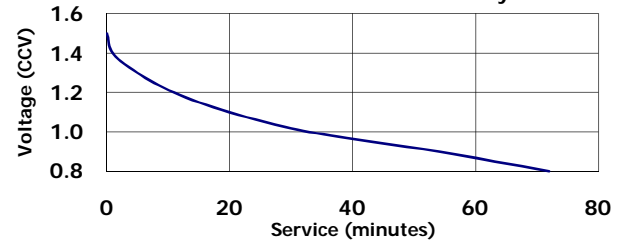
PHOTOFLASH 600 mA 10 sec/min 1 hr/day
