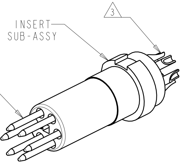
MALE CONTACT
