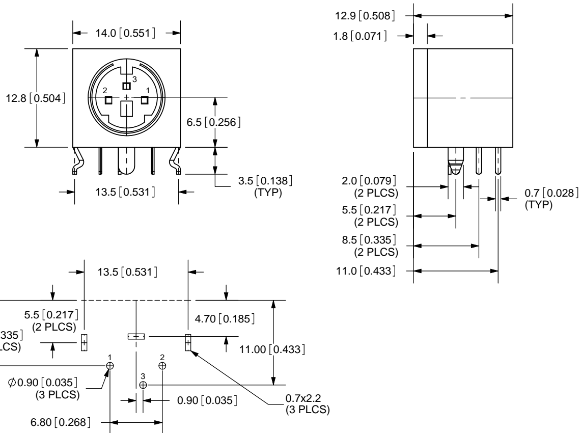
HOLE LAYOUT TOP VIEW
