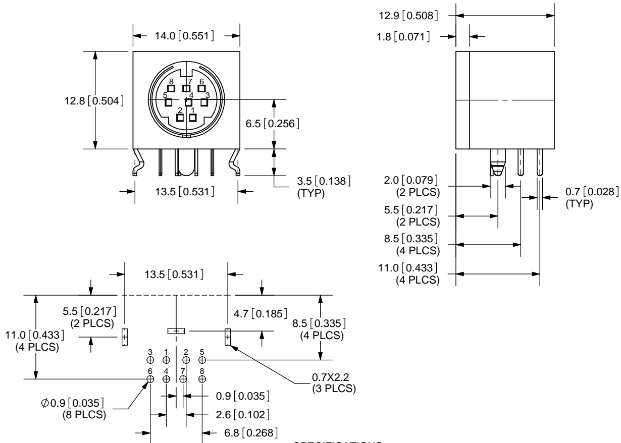
HOLE LAYOUT TOP VIEW
