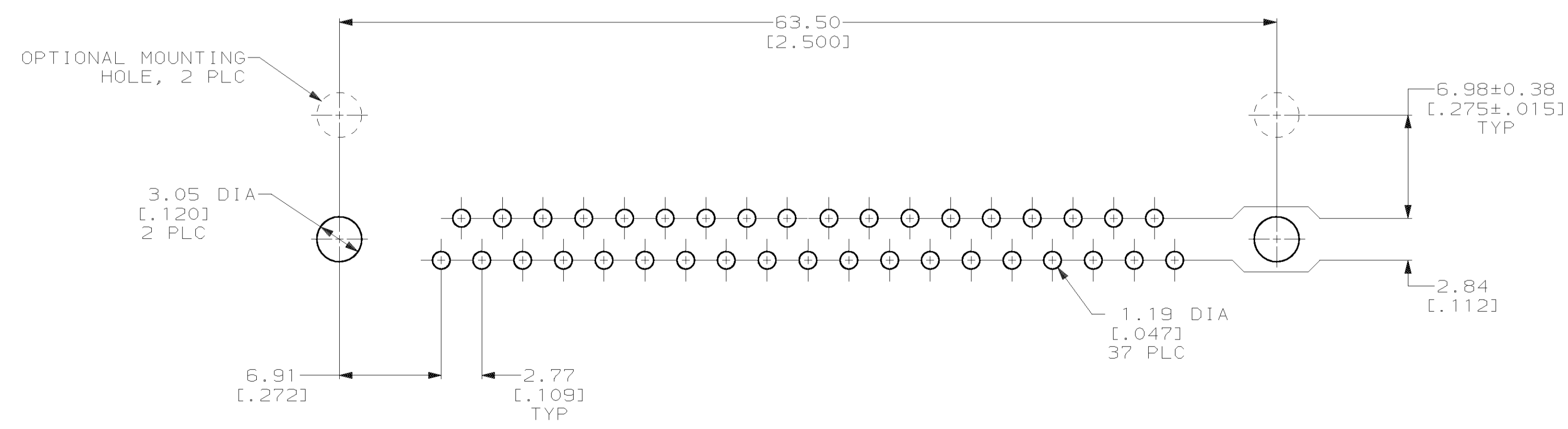
PC BOARD MOUNTING DIMENSIONS
