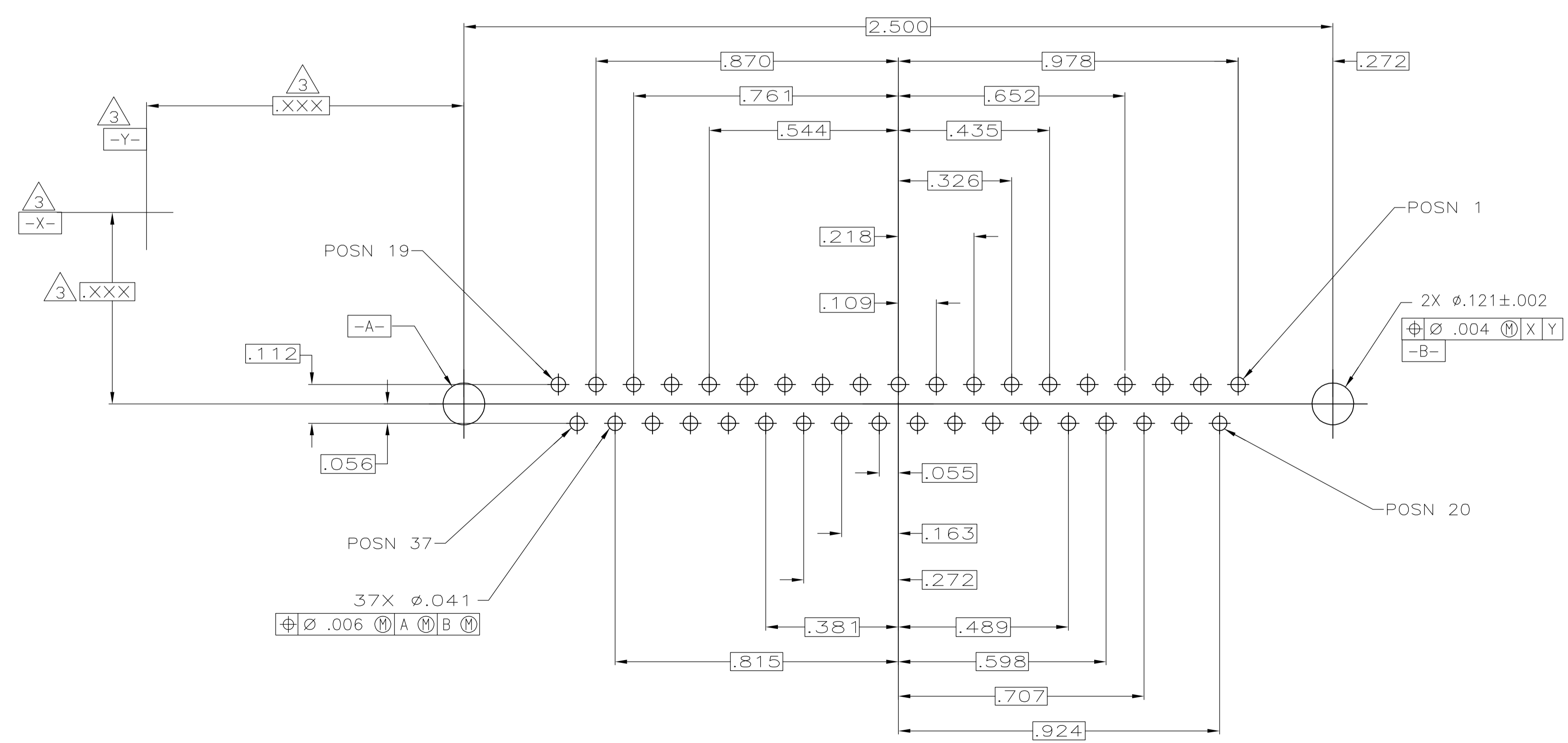
RECOMMENDED PC BOARD MOUNTING DIMENSIONS
