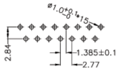
15 Pin Male Connector PCB Pin Layout Scale 2:1
