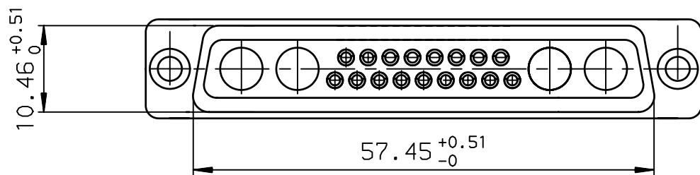
LAYOUT DIMENSIONS (after plating) CONNECTOR SIDE VIEW
