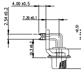
VIEW WITHOUT POWERS CONTACTS
