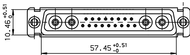
LAYOUT DIMENSIONS (after plating) CONNECTOR SIDE VIEW
