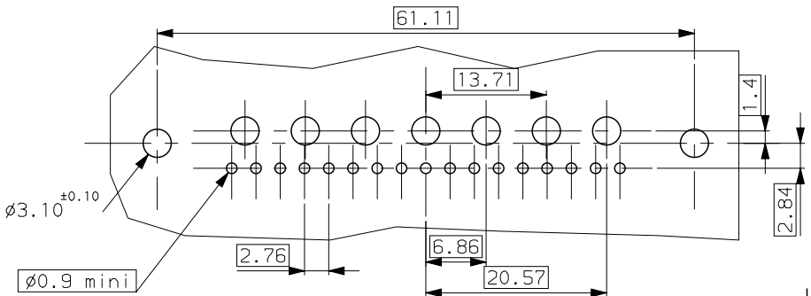
PC CARD drilling dimensions
