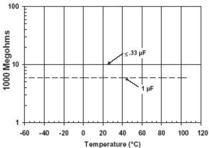
Insulation Resistance
