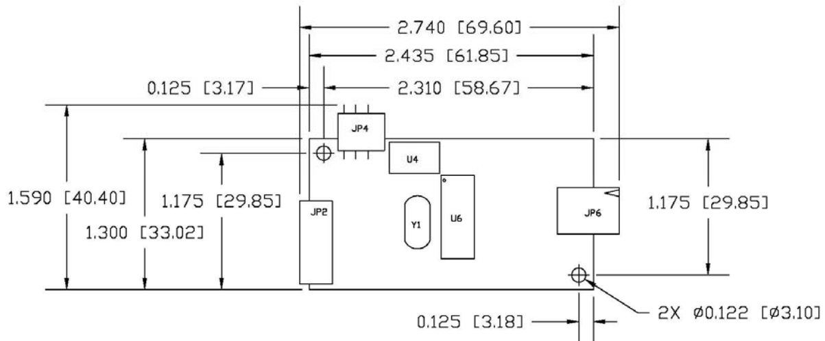
Figure 1. SC400 Overall Dimensions
