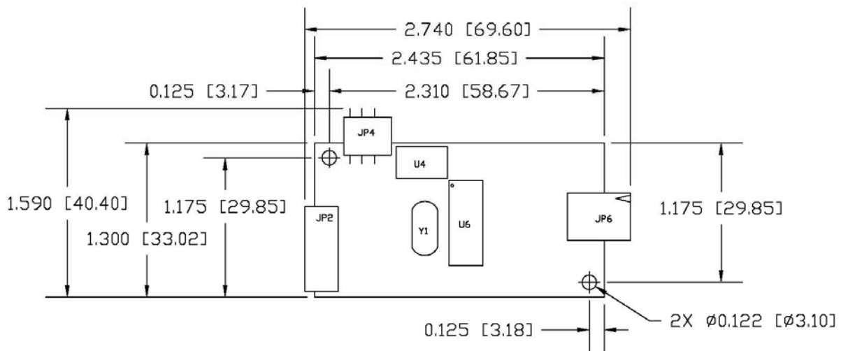
Figure 3 SC400 Touch Screen Controller
