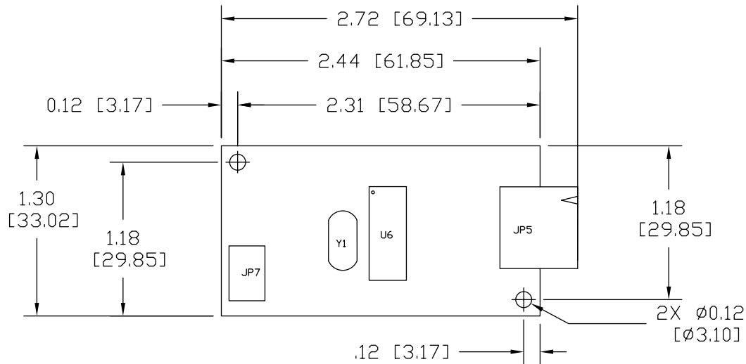
Figure 1. SC800 USB Controller Overall Dimensions
