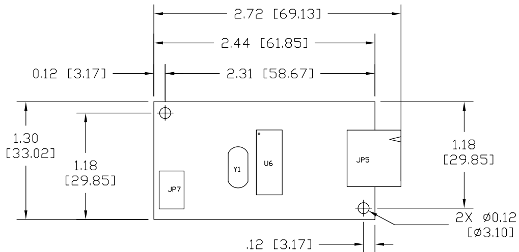
Figure 3. SC800 USB Touch Screen Controller Dimensions
