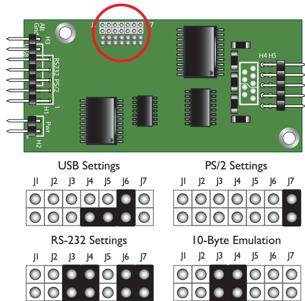
Communication Jumper Settings
