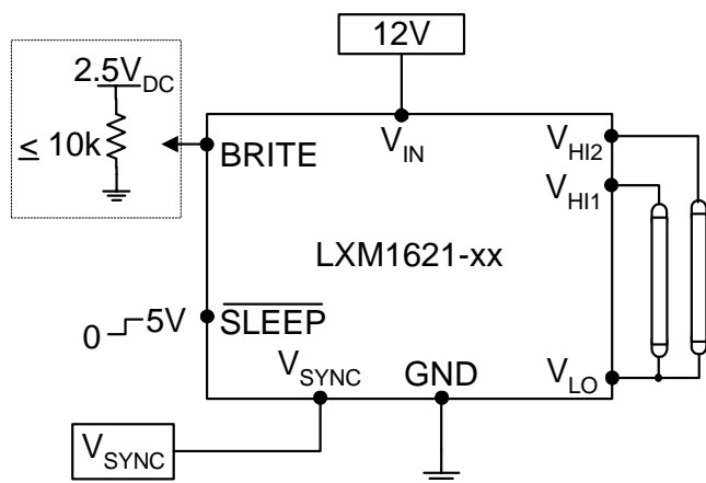
Figure 7- Brightness Control
