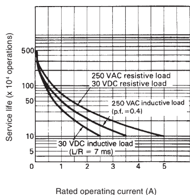
One pole
