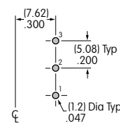
Single Pole
