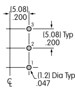
Single Pole
