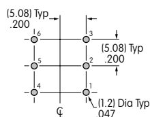
Double Pole
