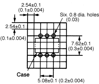
Mounting holes PCB dimension (Top view)
