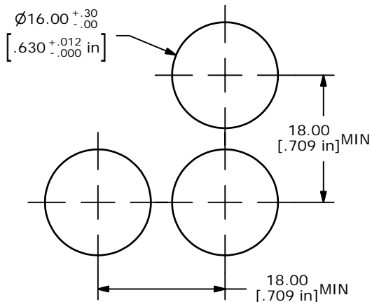
PANEL MOUNTING.
