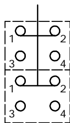
DPDT CONTACT CONFIGURATION
