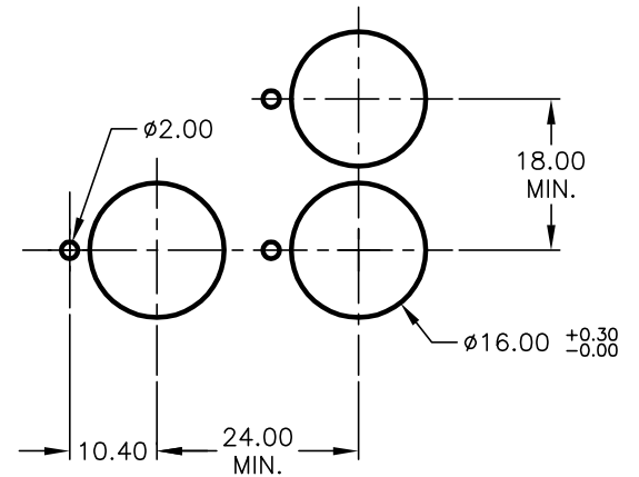
RECOMMENDED PANEL MOUNTING SCALE 1:1
