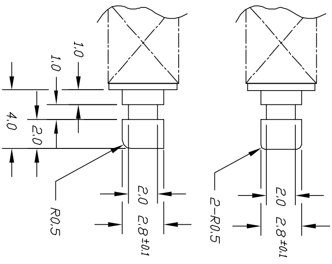
ACTUATOR DETAIL SCALE 4:1
