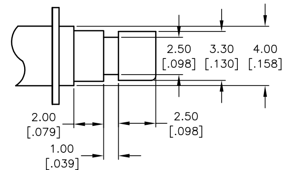
(ACTUATOR DETAIL) SCALE 4:1
