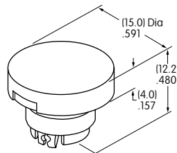
AT3002 Round
