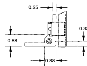
Hinge Detail
