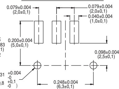
CARRIER TAPE
