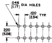
RECOMMENDED PC BOARD LAYOUT (Component Side)
