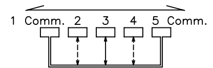
CIRCUIT:SP3T CONTACT CONFIGURATION
