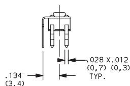
ESD PIN WITH PTS453TL38 MODEL ONLY
