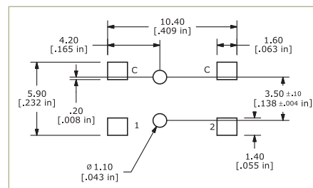
P.C. MOUNTING
