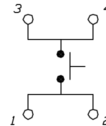
CIRCUIT: SPST
