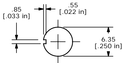
PANEL MOUNTING
