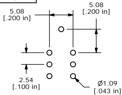
P.C. MOUNTING
