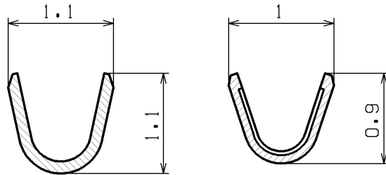
INSULATION BARREL (Y-Y sec.)
