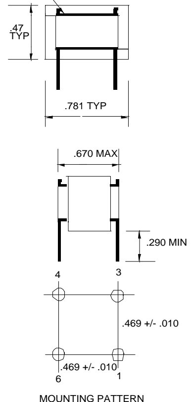
MOUNTING PATTERN
